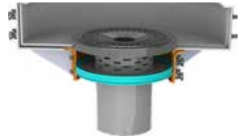
Upper Katch Kan™ attached to Surface Junk Basket™ with Window Stripper™ inside.
